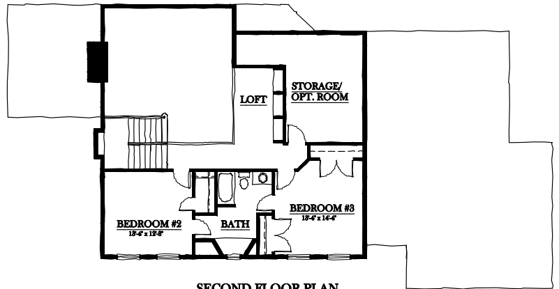
SECOND FLOOR PLAN 752 SF.
