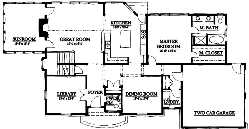
FIRST FLOOR PLAN 1,945 SF.
